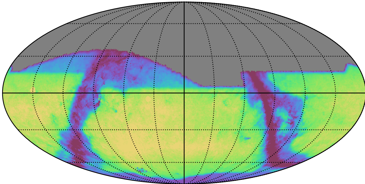
weather_cloudso36v3.5_10yrs i: GalaxyCountsMetricExtended
