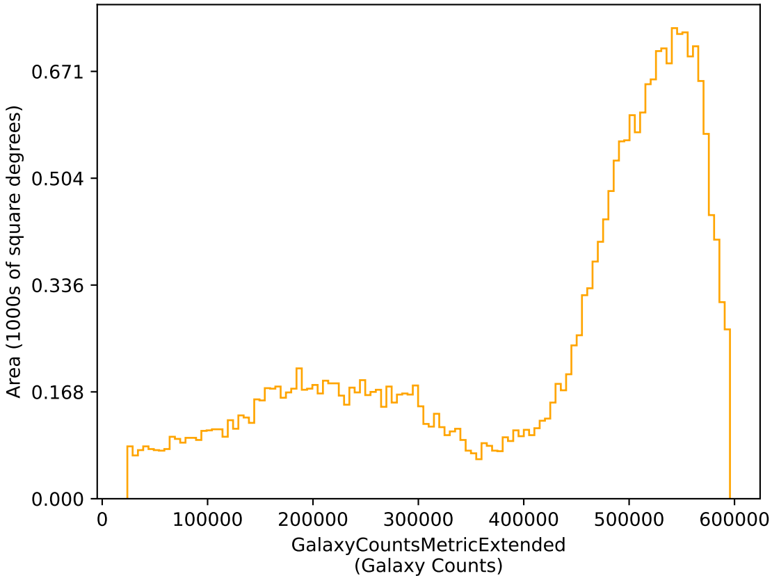
weather_cloudso36v3.5_10yrs r: GalaxyCountsMetricExtended
