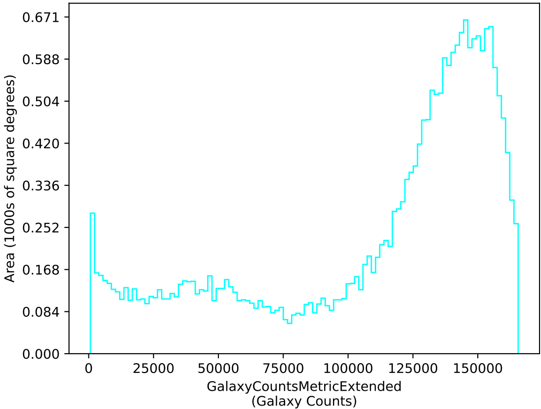
weather_cloudso36v3.5_10yrs u: GalaxyCountsMetricExtended
