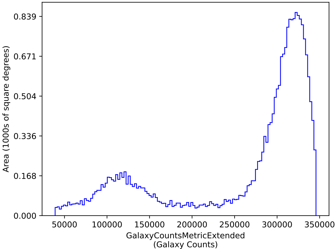
weather_cloudso36v3.5_10yrs y: GalaxyCountsMetricExtended
