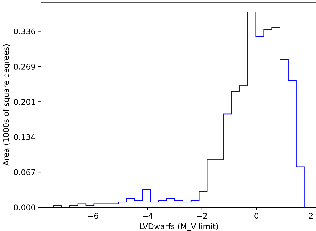
weather_cloudso36v3.5_10yrs gi SCP: LVDwarfs
