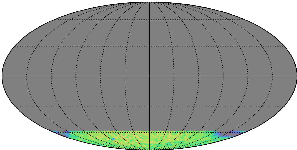
weather_cloudso36v3.5_10yrs gi SCP: LVDwarfs
