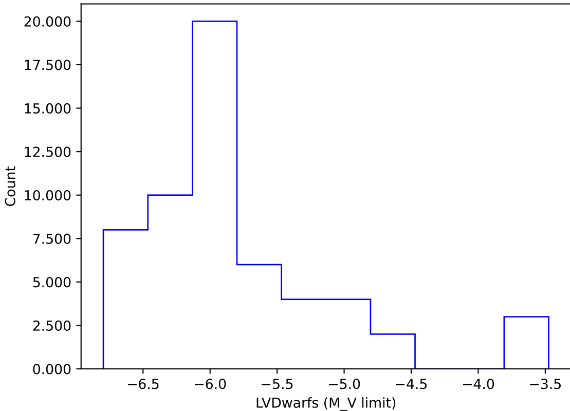
weather_cloudso36v3.5_10yrs gi: LVDwarfs
