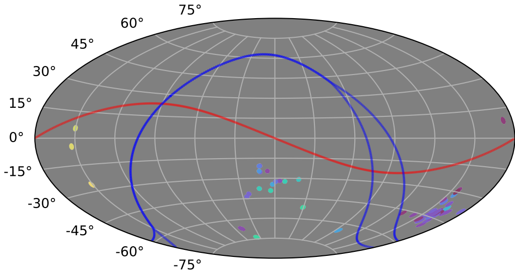
weather_cloudso36v3.5_10yrs gi: LVDwarfs
