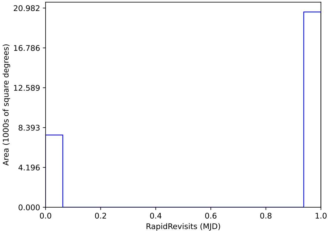
weather_cloudso36v3.5_10yrs : RapidRevisits
