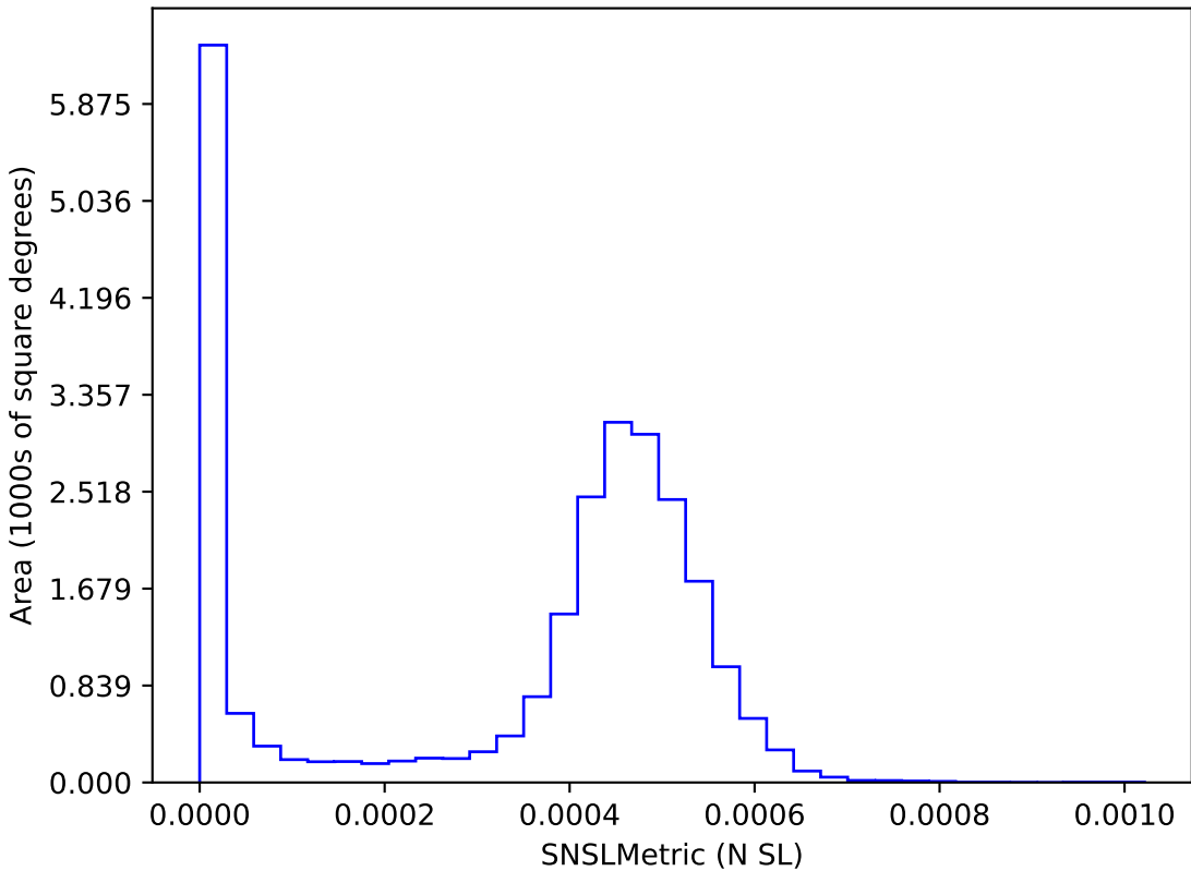
weather_cloudso36v3.5_10yrs : SNSLMetric
