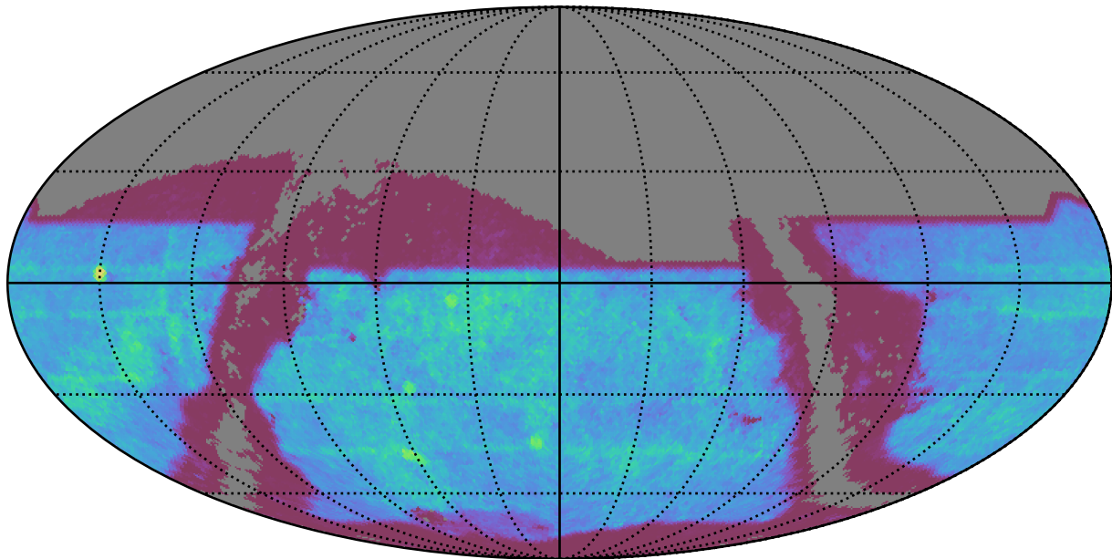
weather_cloudso36v3.5_10yrs : SNSLMetric
