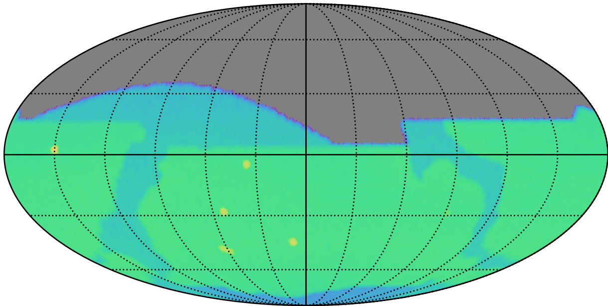
weather_cloudso36v3.5_10yrs r: SurfaceBrightLimit
