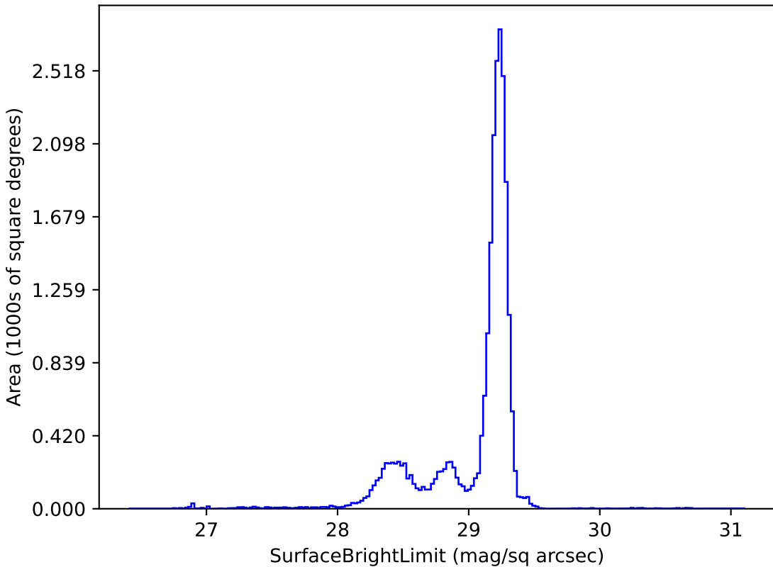
weather_cloudso36v3.5_10yrs u: SurfaceBrightLimit
