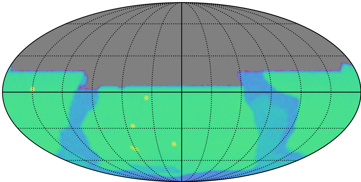
weather_cloudso36v3.5_10yrs y: SurfaceBrightLimit
