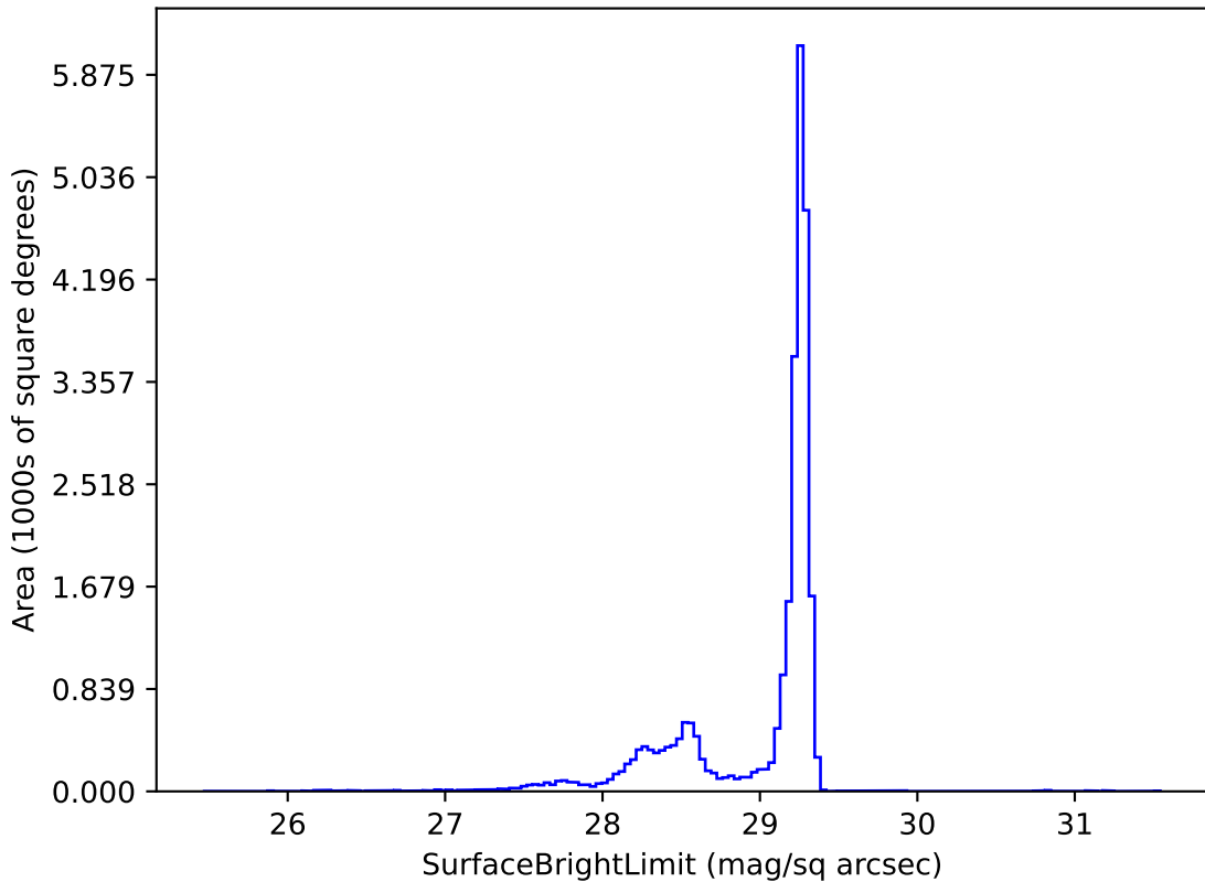
weather_cloudso36v3.5_10yrs z: SurfaceBrightLimit
