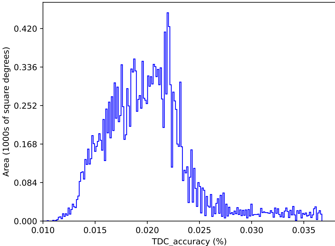
weather_cloudso36v3.5_10yrs : TDC_accuracy
