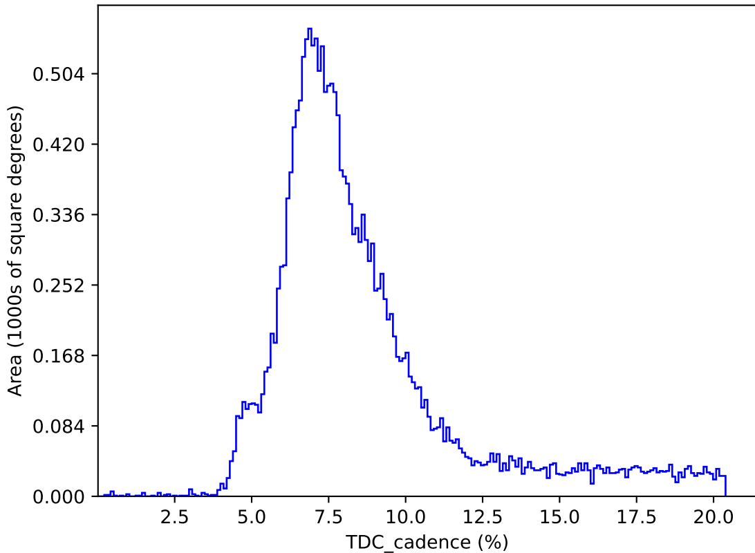
weather_cloudso36v3.5_10yrs : TDC_cadence
