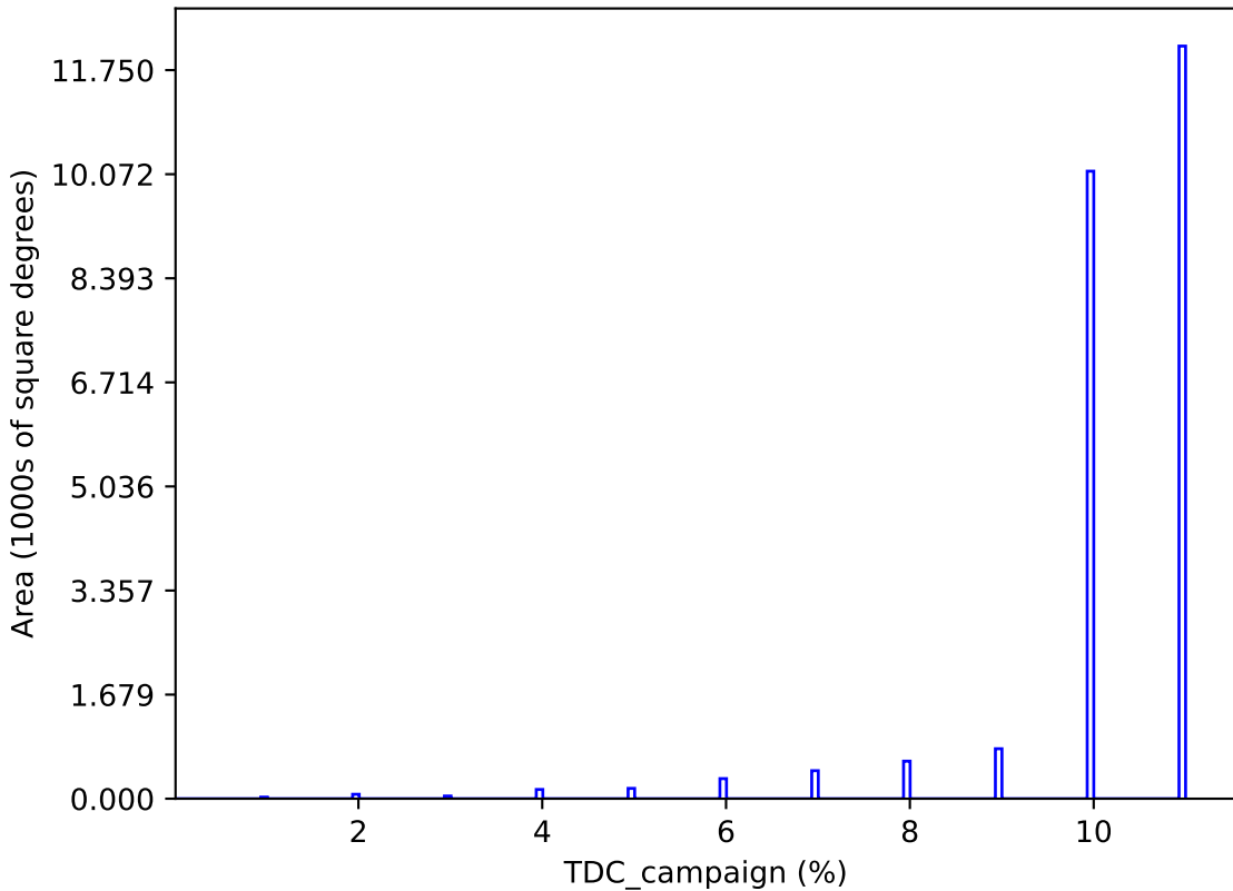
weather_cloudso36v3.5_10yrs : TDC_campaign
