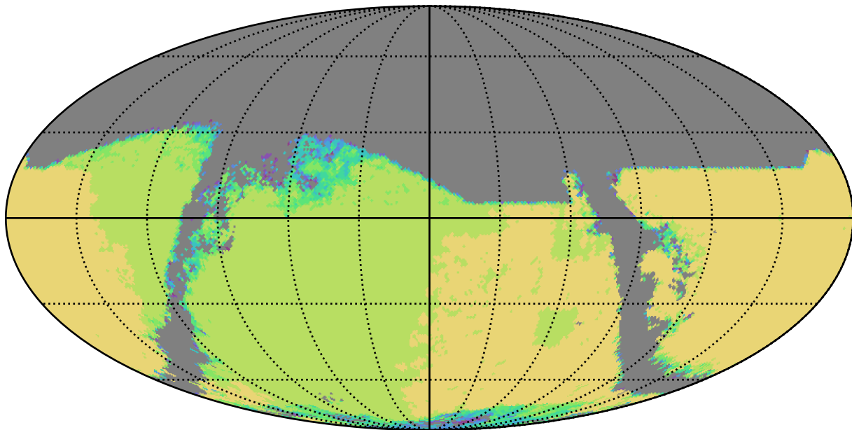
weather_cloudso36v3.5_10yrs : TDC_campaign
