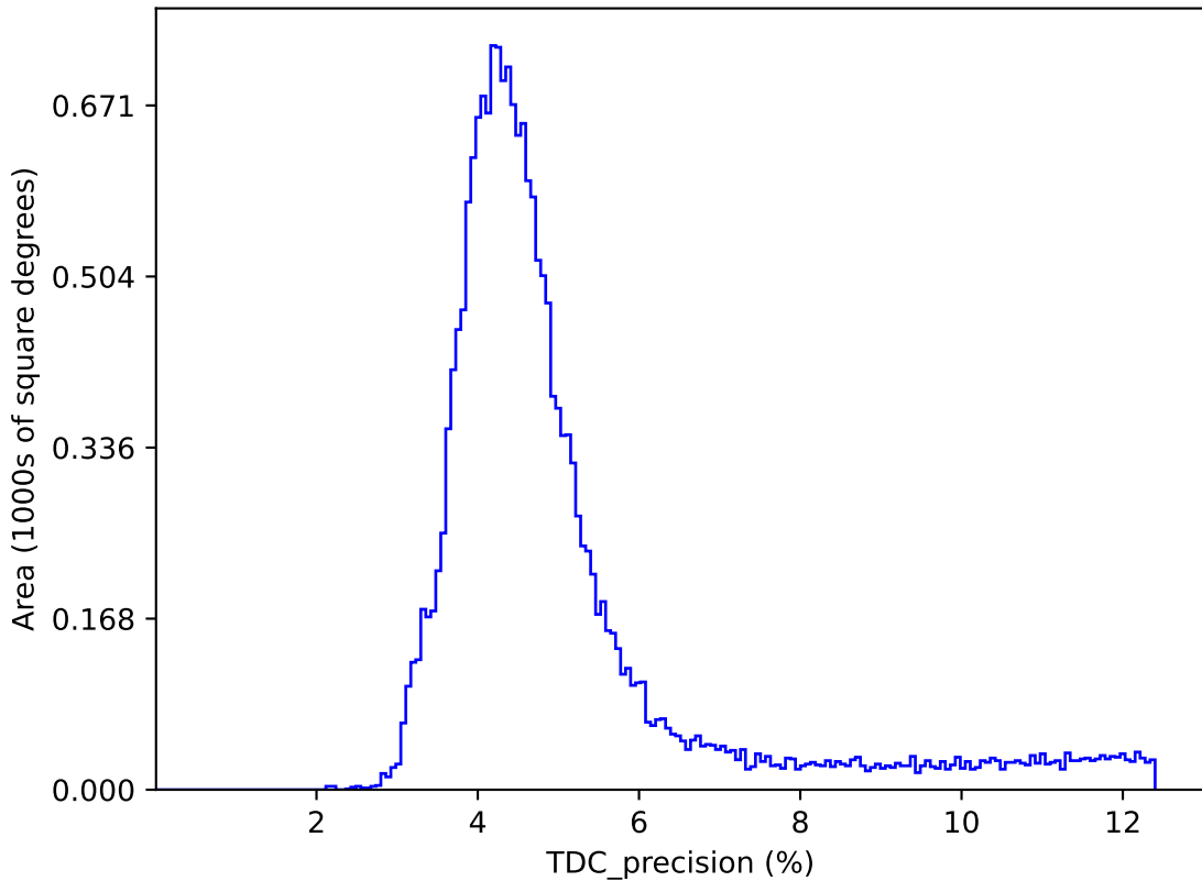
weather_cloudso36v3.5_10yrs : TDC_precision
