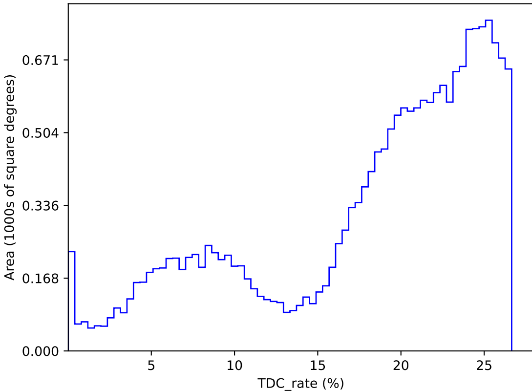
weather_cloudso36v3.5_10yrs : TDC_rate
