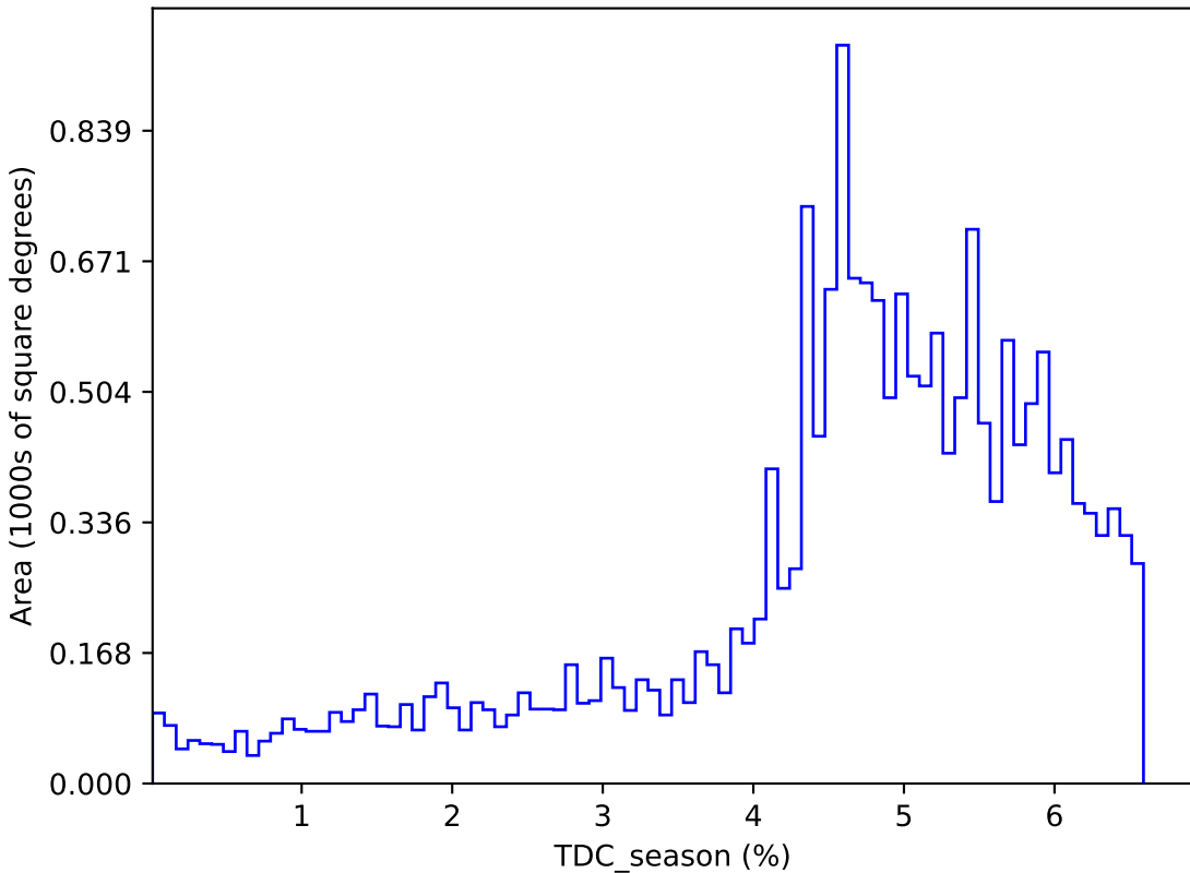
weather_cloudso36v3.5_10yrs : TDC_season
