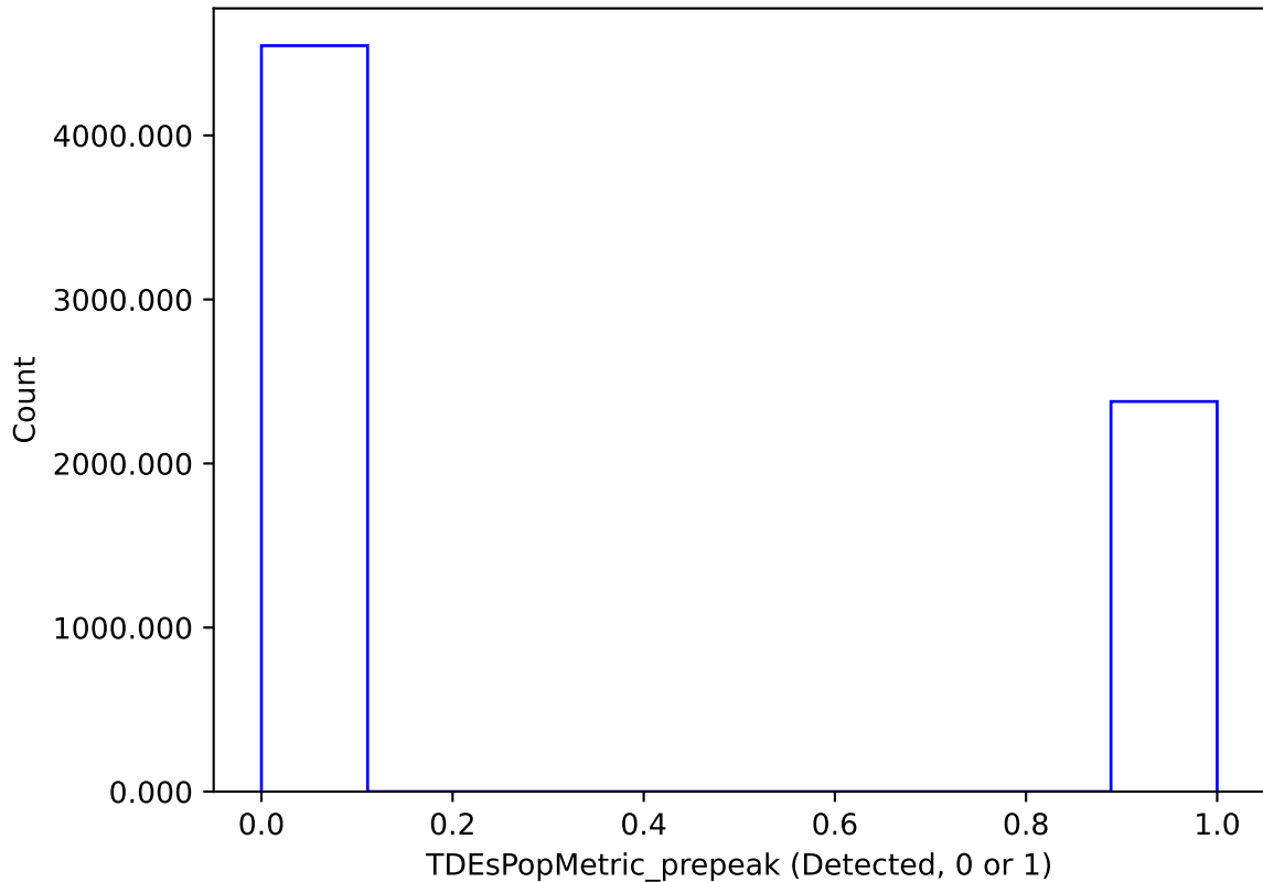
weather_cloudso36v3.5_10yrs : TDEsPopMetric_prepeak
