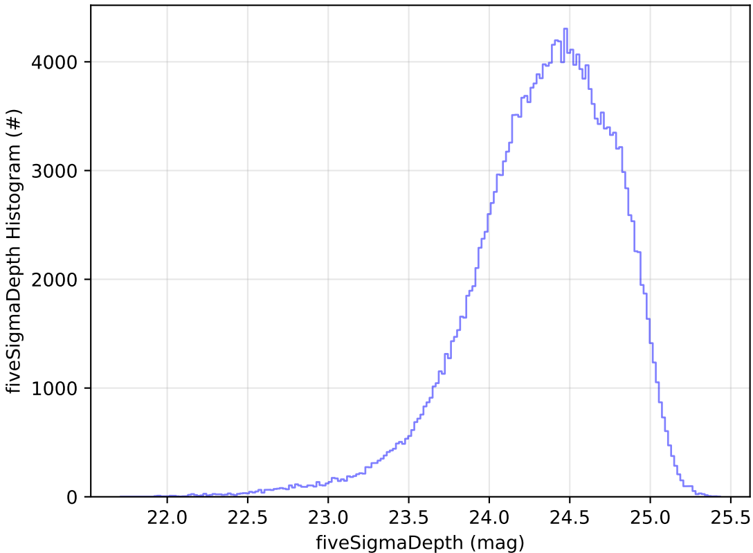
weather_cloudso36v3.5_10yrs g: fiveSigmaDepth Histogram
