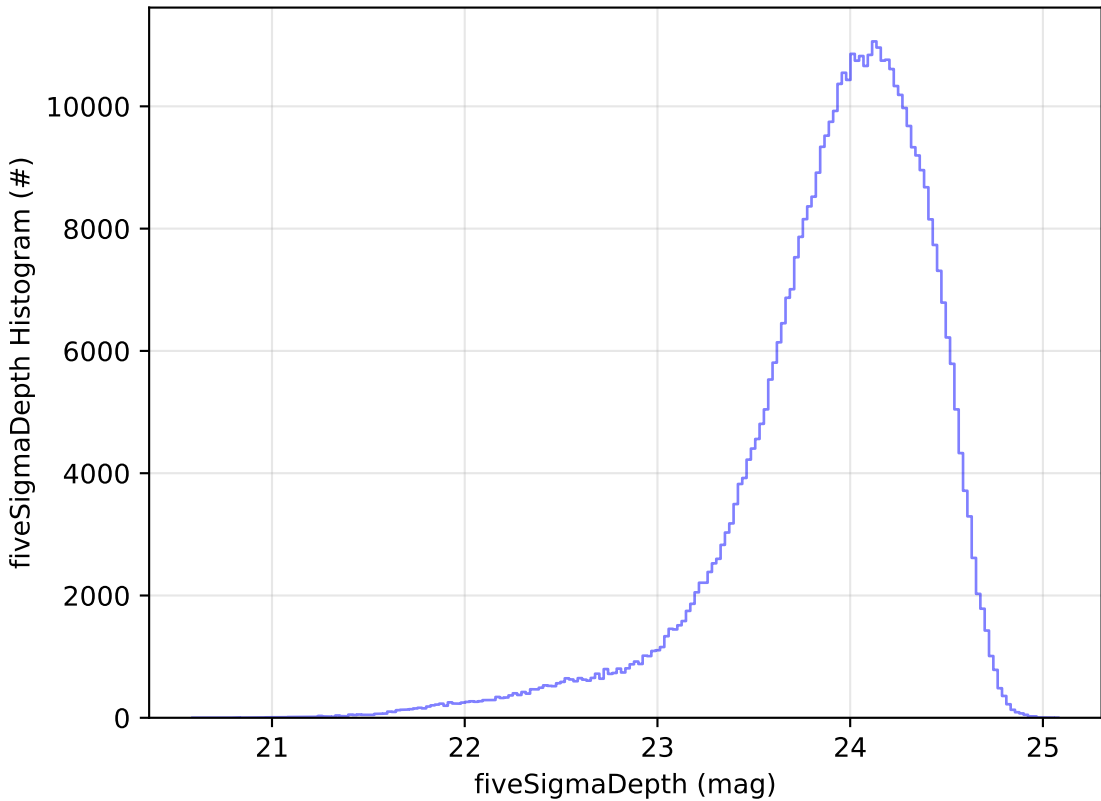
weather_cloudso36v3.5_10yrs r: fiveSigmaDepth Histogram
