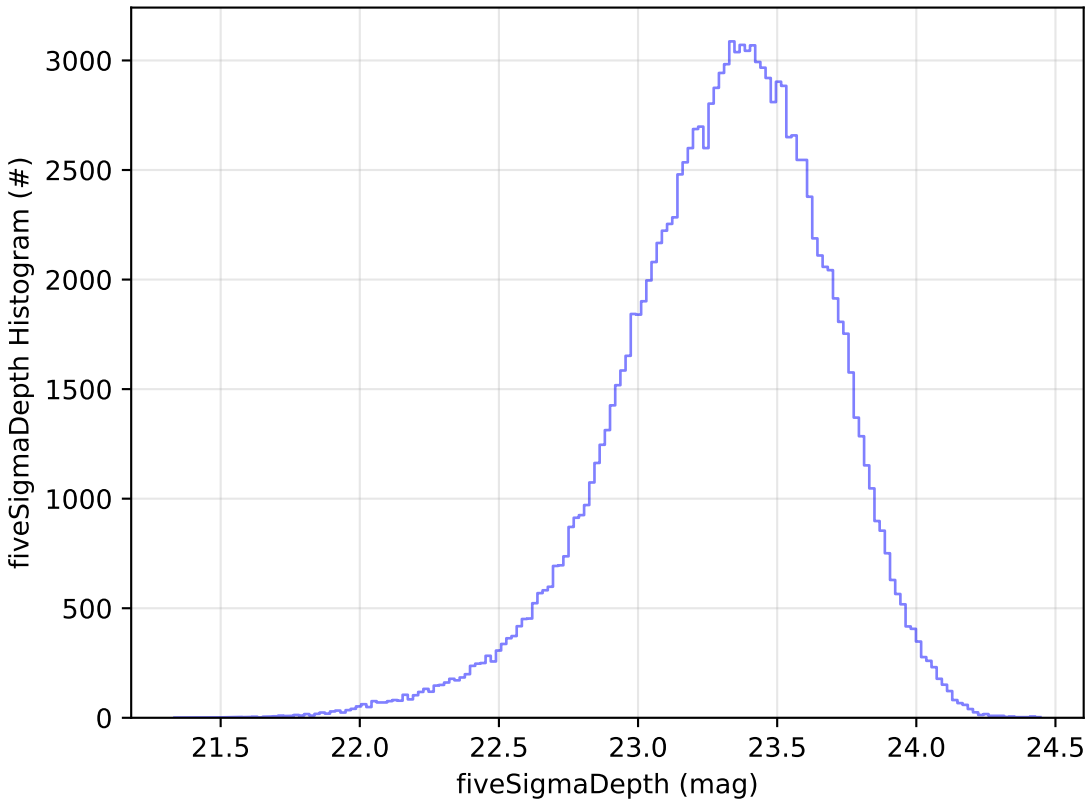
weather_cloudso36v3.5_10yrs u: fiveSigmaDepth Histogram
