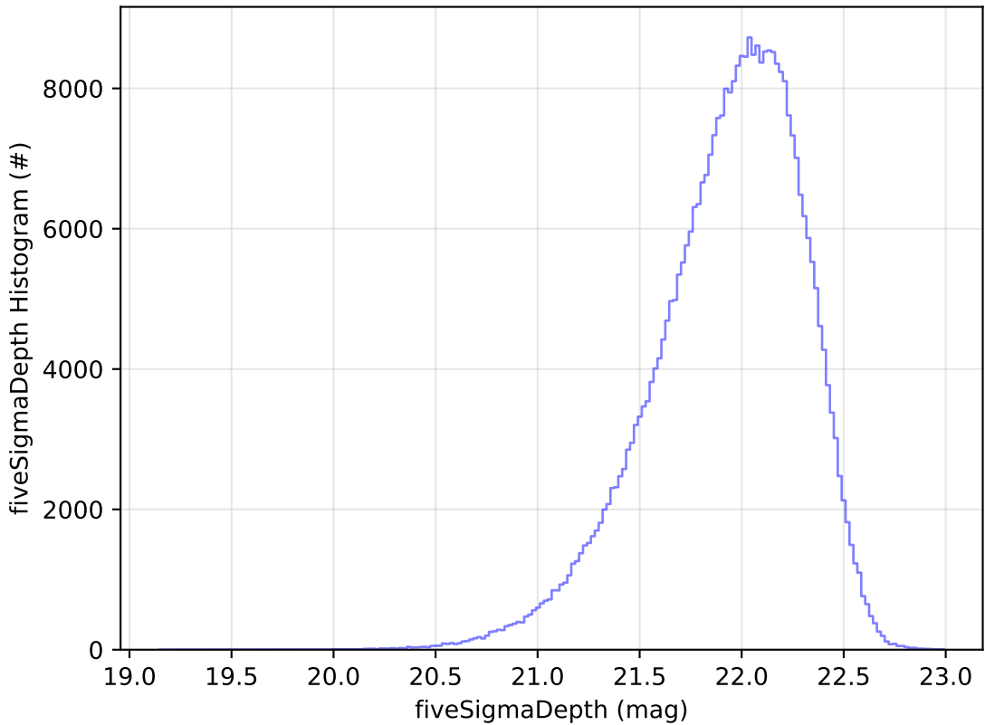
weather_cloudso36v3.5_10yrs y: fiveSigmaDepth Histogram
