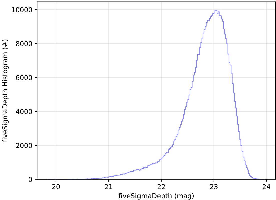
weather_cloudso36v3.5_10yrs z: fiveSigmaDepth Histogram
