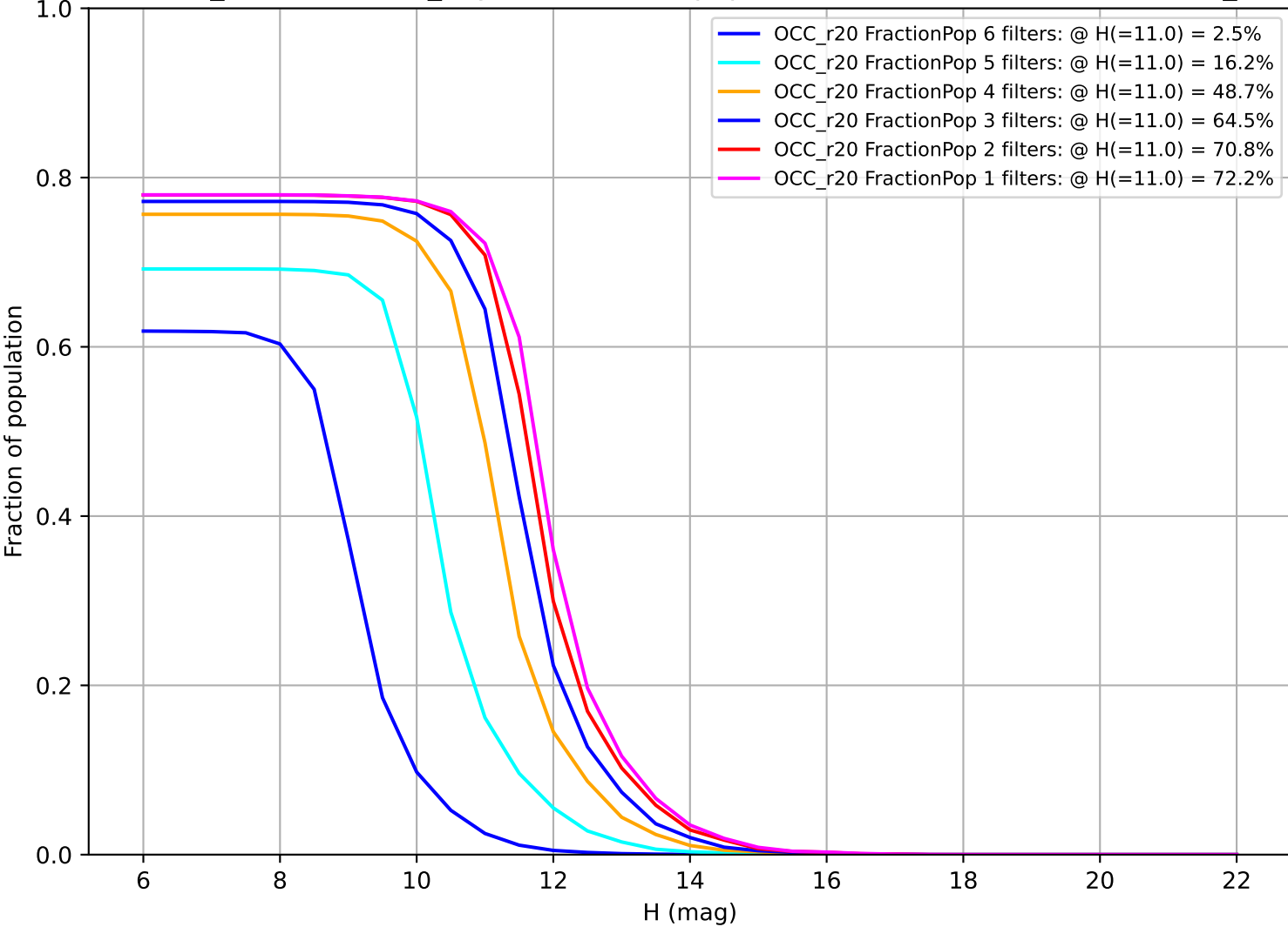
weather_cloudso36v3.5_10yrs: Fraction of population with colors in X filters OCC_r20
