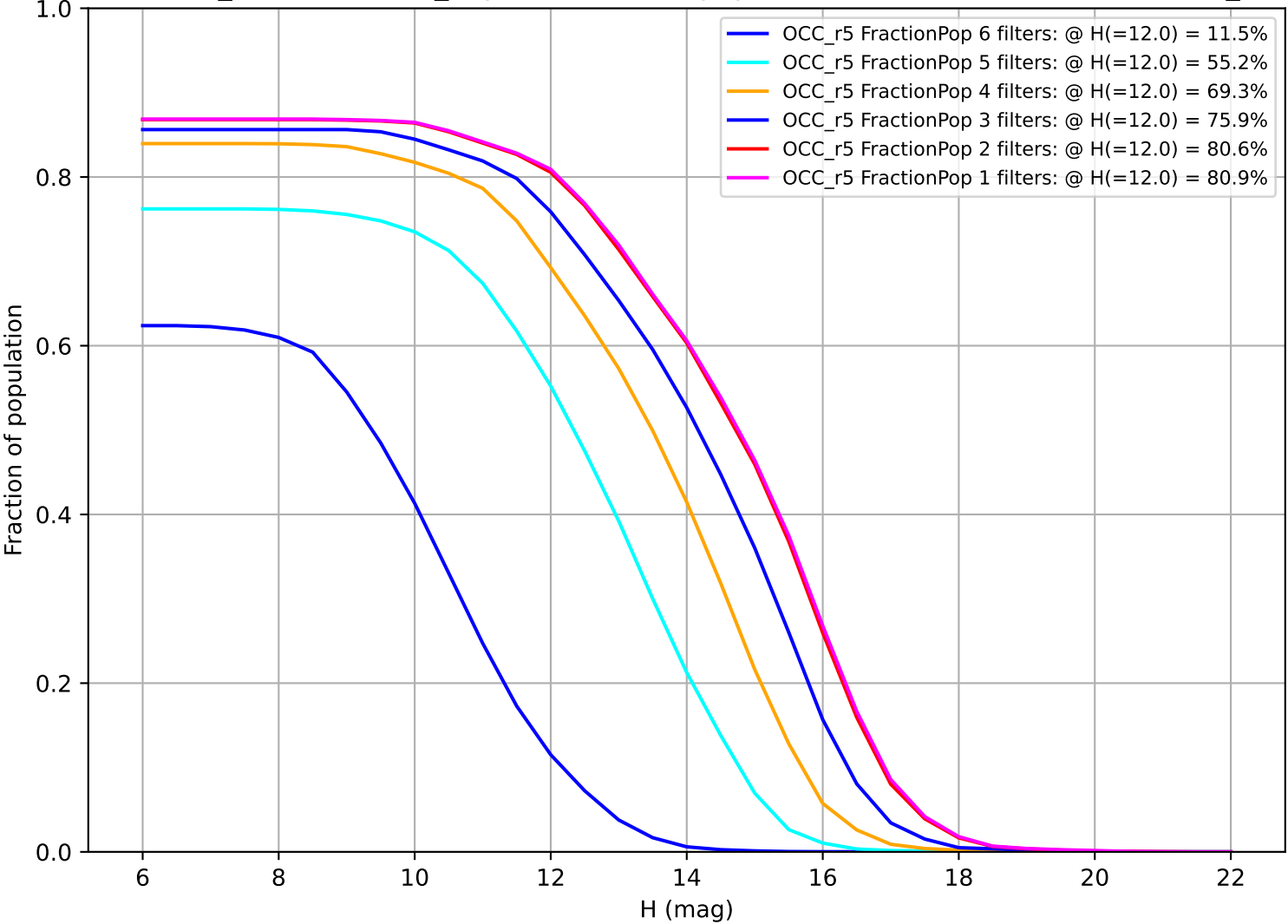
weather_cloudso36v3.5_10yrs: Fraction of population with colors in X filters OCC_r5
