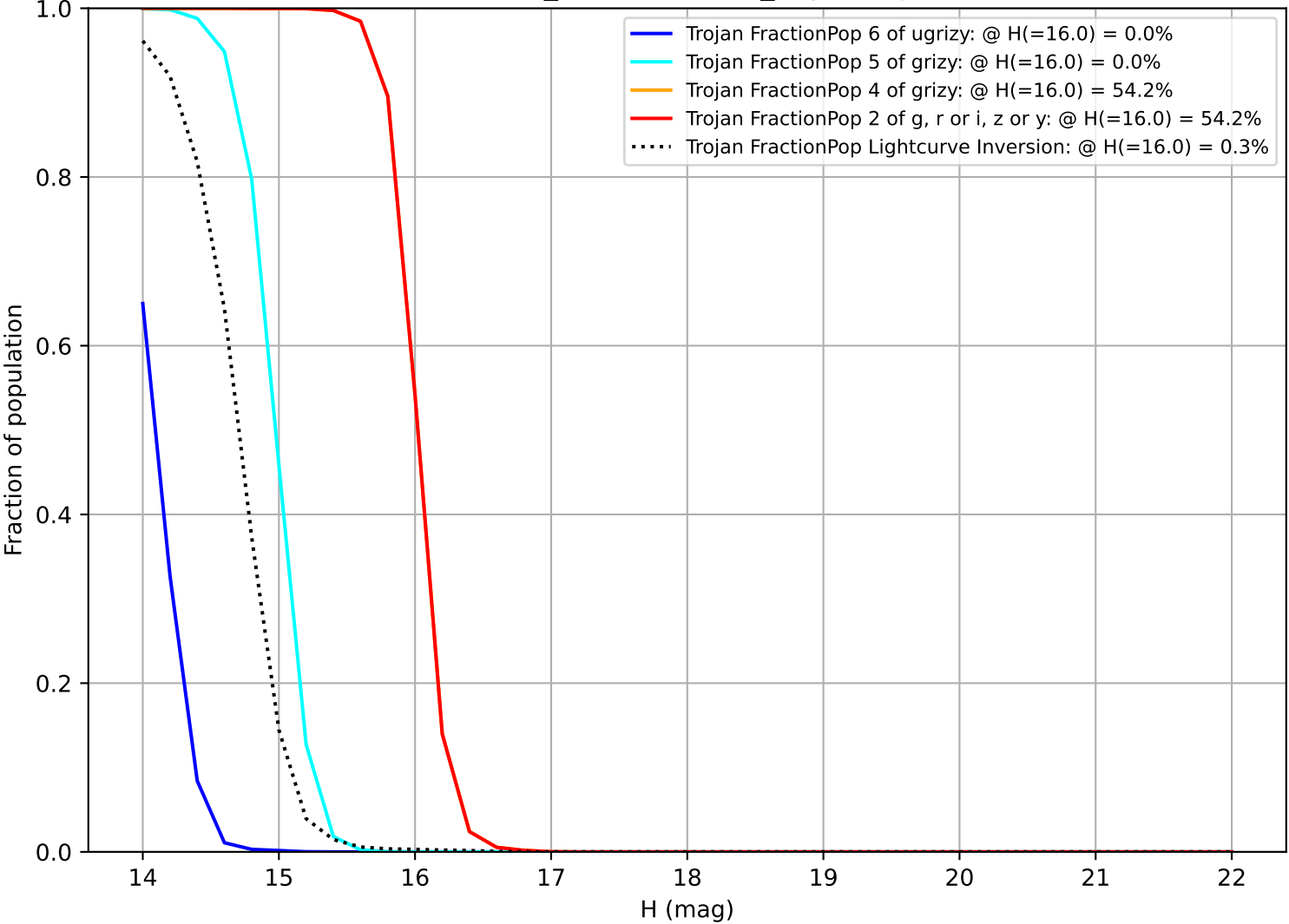
weather_cloudso36v3.5_10yrs Trojan
