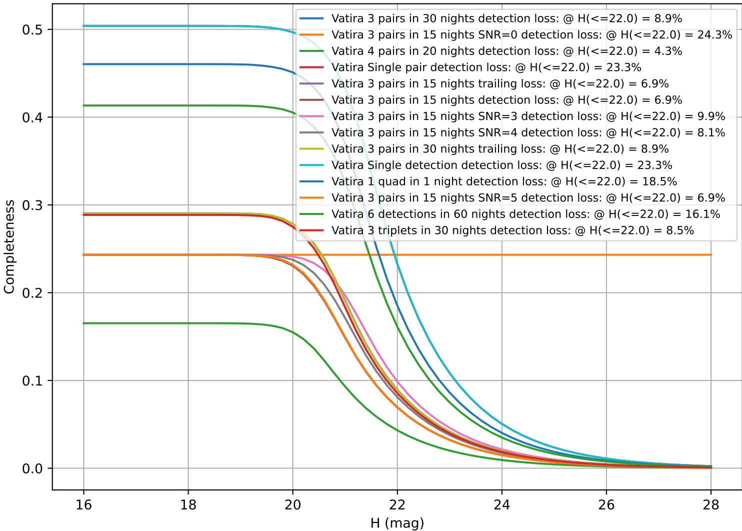
weather_cloudso36v3.5_10yrs: CumulativeCompleteness
