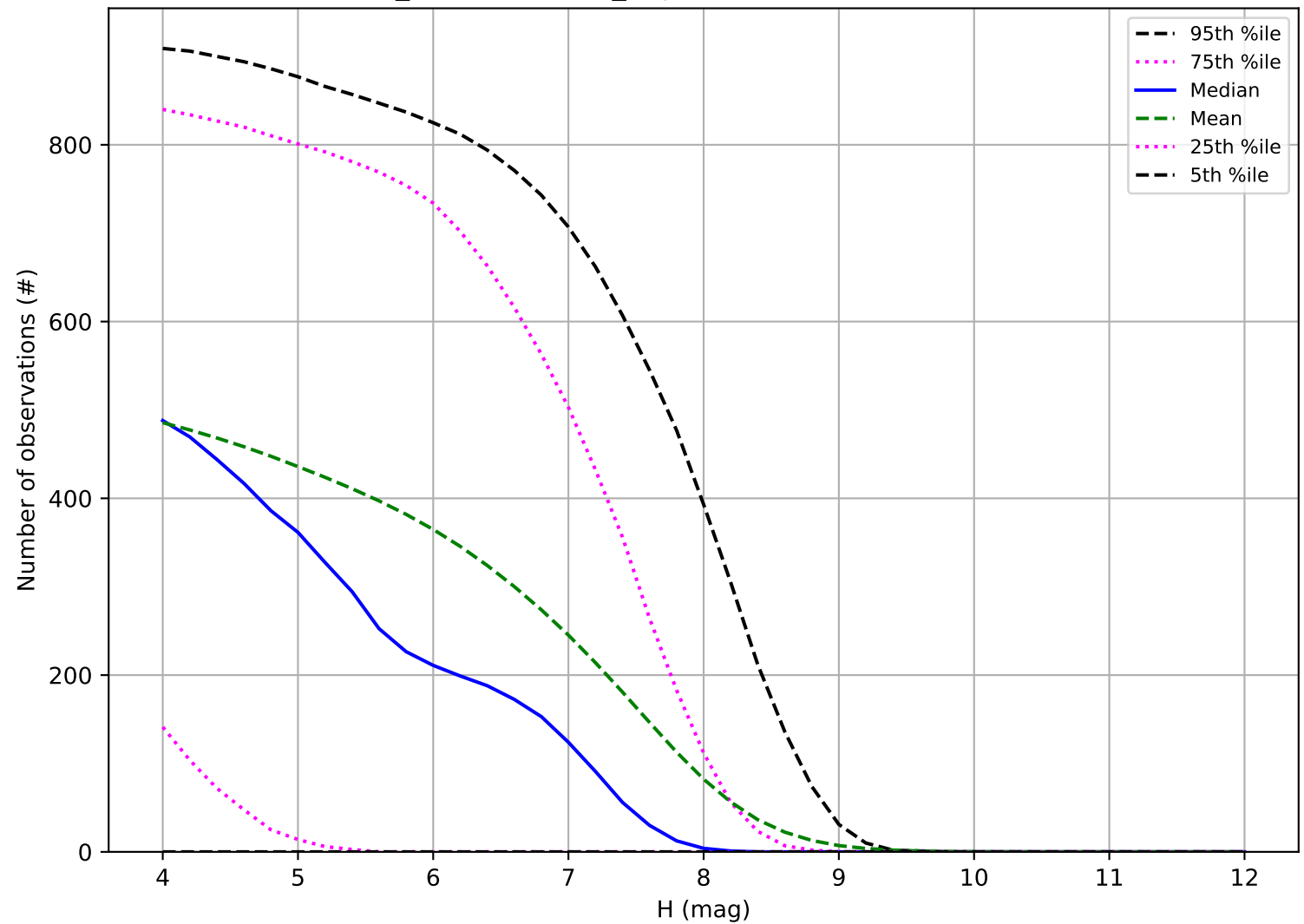
weather_cloudso36v3.5_10yrs: Number of observations TNO
