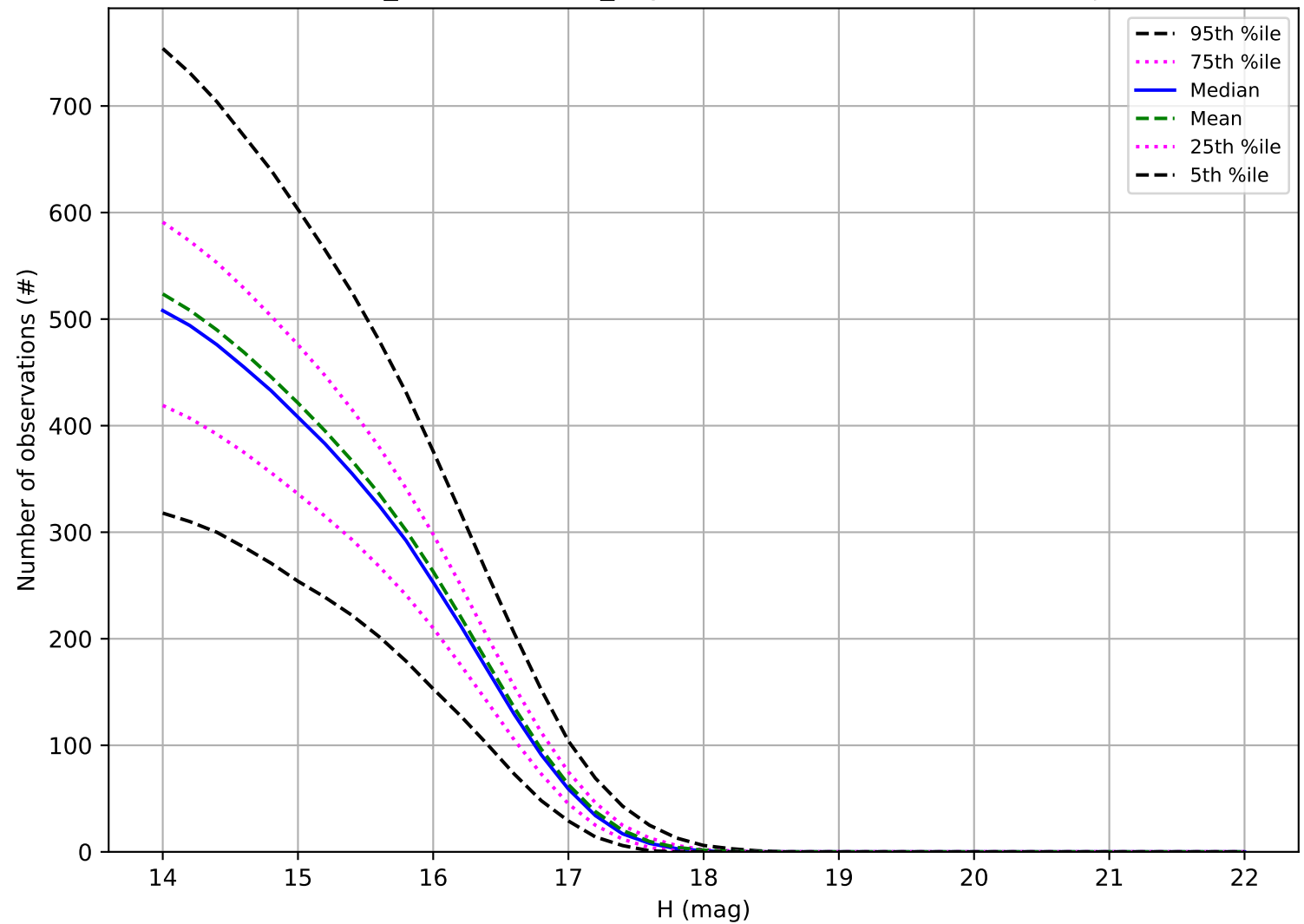
weather_cloudso36v3.5_10yrs: Number of observations Trojan
