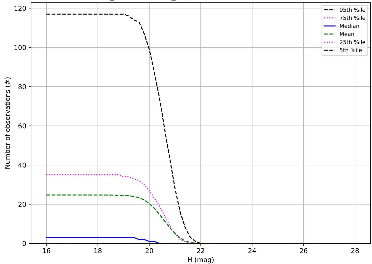
weather_cloudso36v3.5_10yrs: Number of observations Vatira
