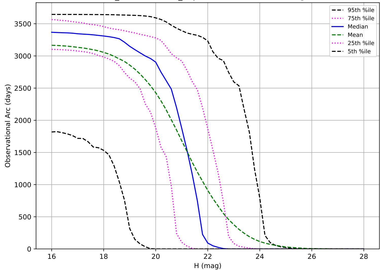
weather_cloudso36v3.5_10yrs: Observational Arc Length NEO
