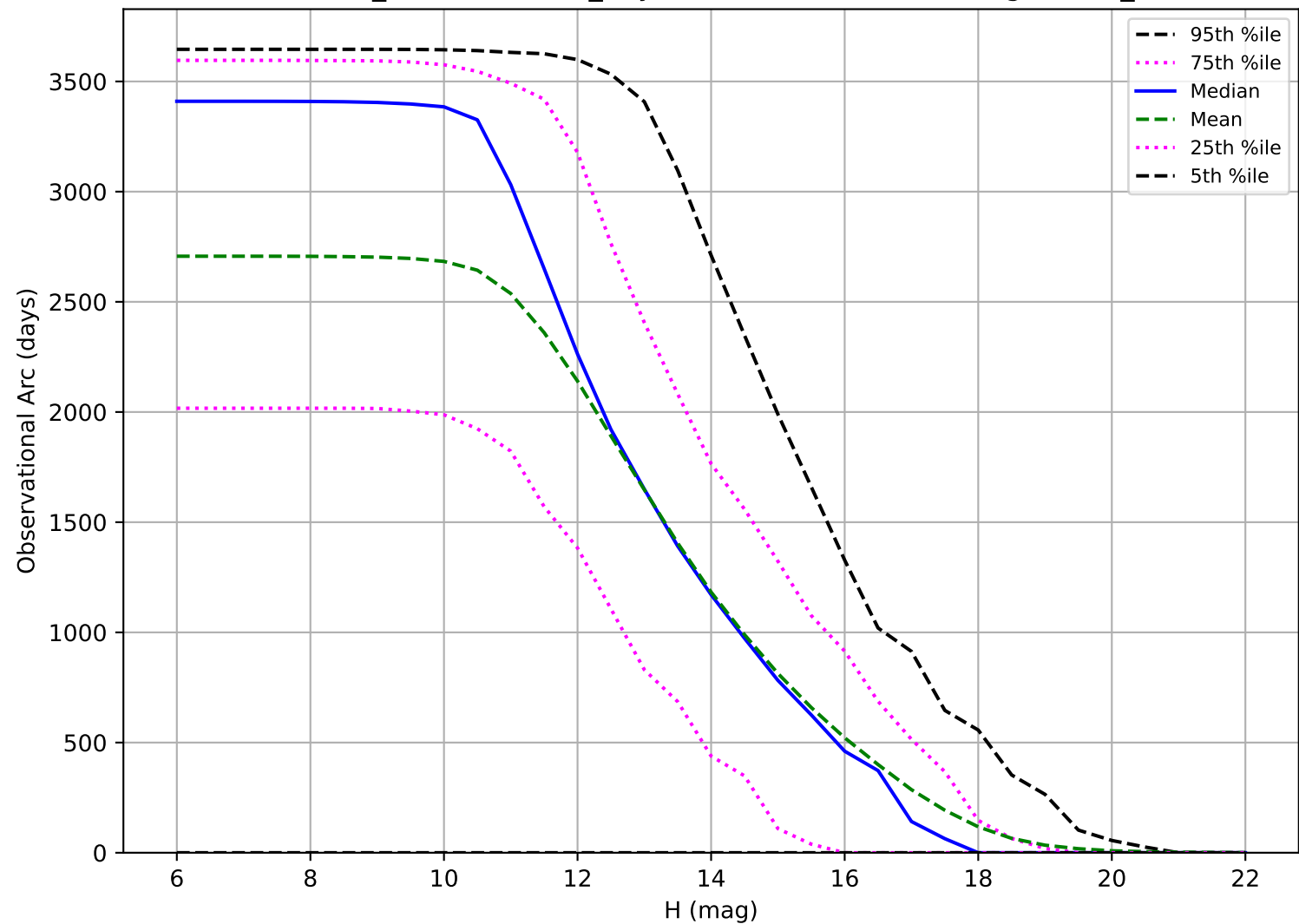
weather_cloudso36v3.5_10yrs: Observational Arc Length OCC_r5
