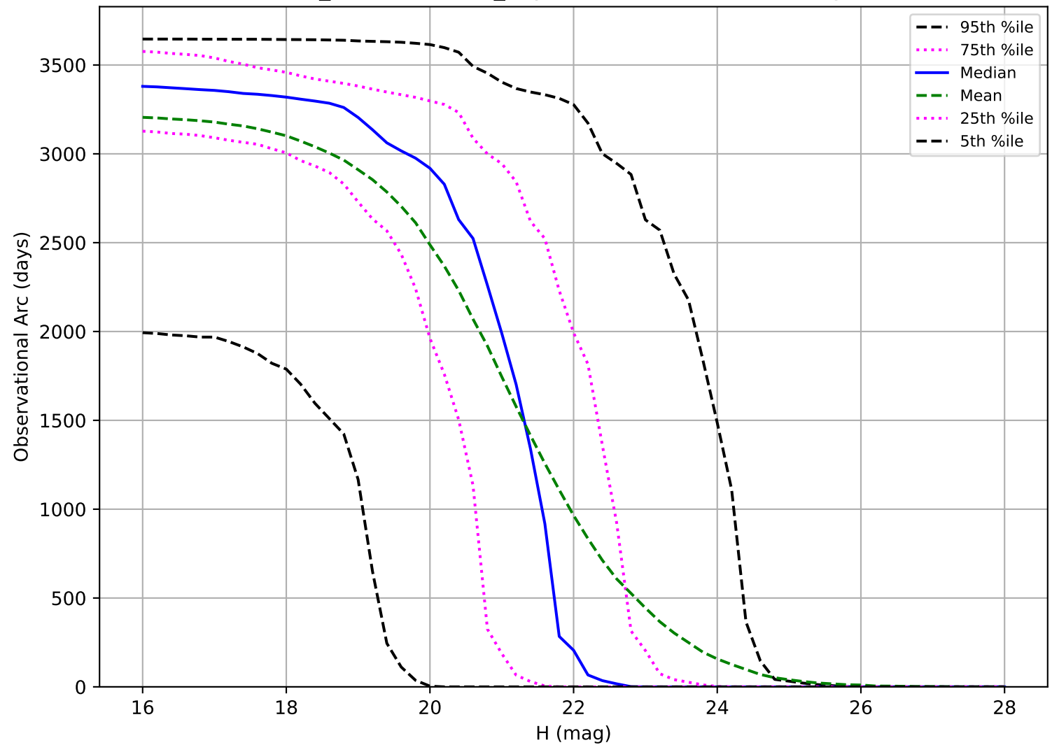
weather_cloudso36v3.5_10yrs: Observational Arc Length PHA
