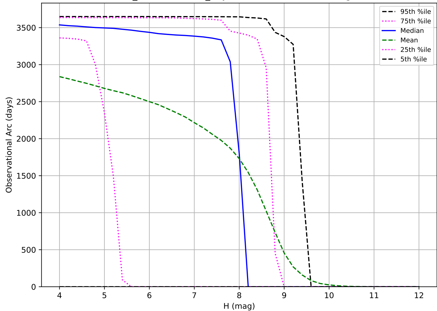
weather_cloudso36v3.5_10yrs: Observational Arc Length TNO
