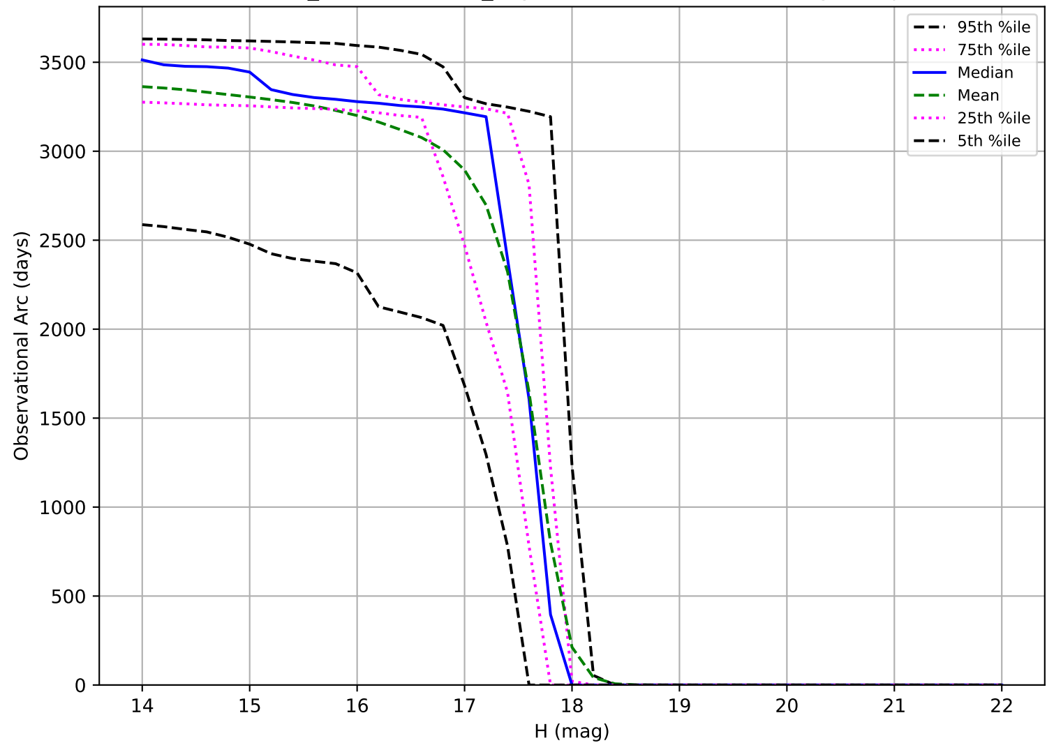
weather_cloudso36v3.5_10yrs: Observational Arc Length Trojan
