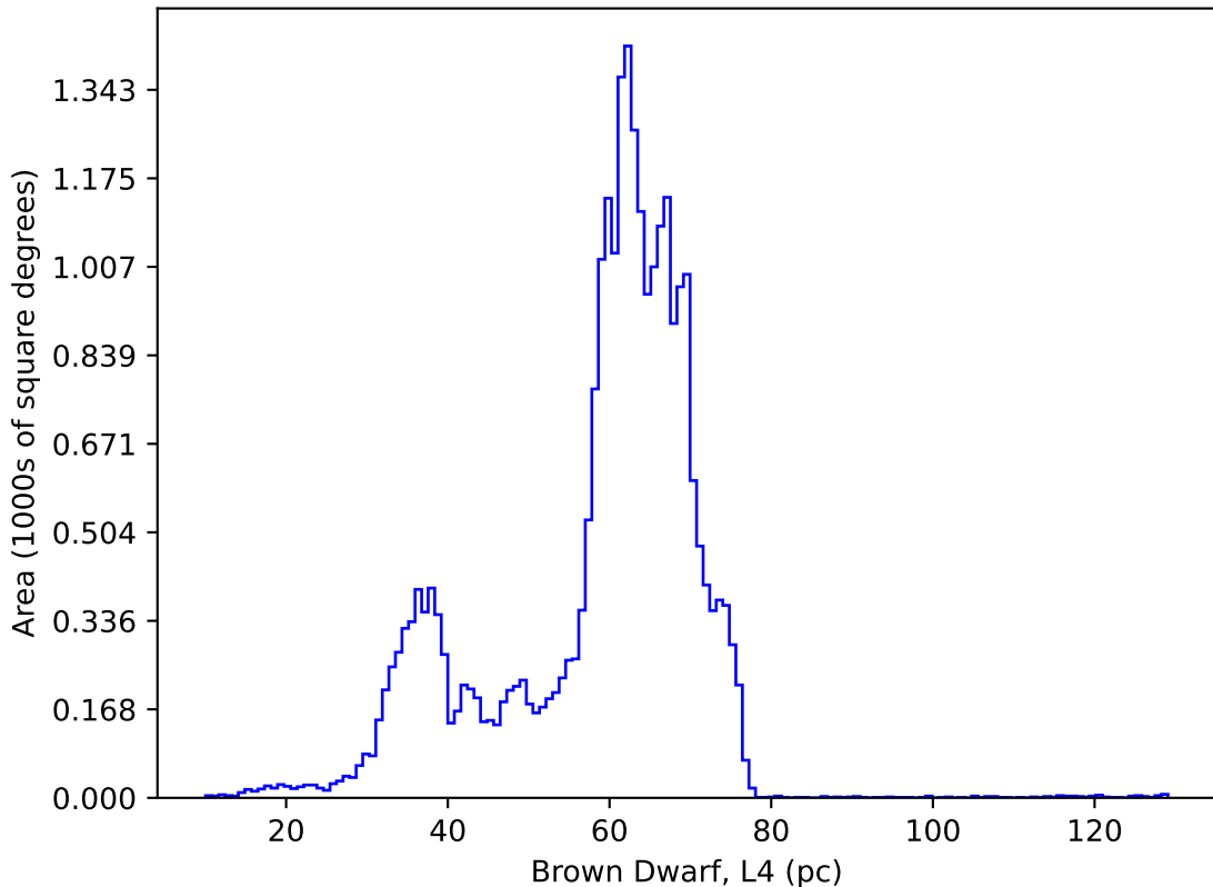
weather_cloudso4v3.5_10yrs : Brown Dwarf, L4
