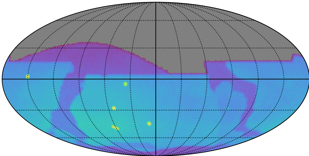
weather_cloudso4v3.5_10yrs : Brown Dwarf, L4
