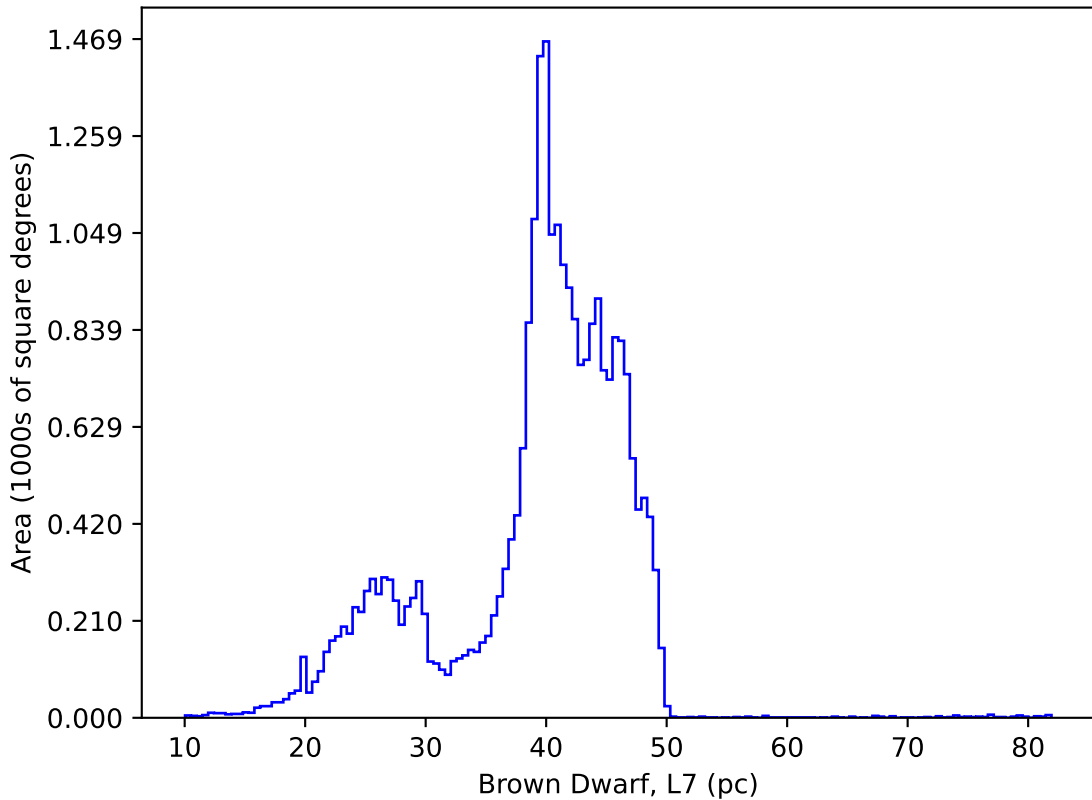
weather_cloudso4v3.5_10yrs : Brown Dwarf, L7
