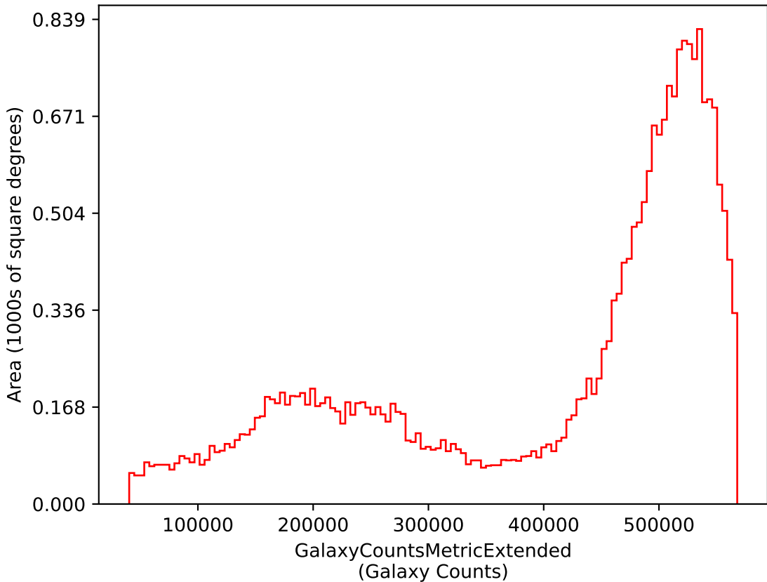
weather_cloudso4v3.5_10yrs i: GalaxyCountsMetricExtended
