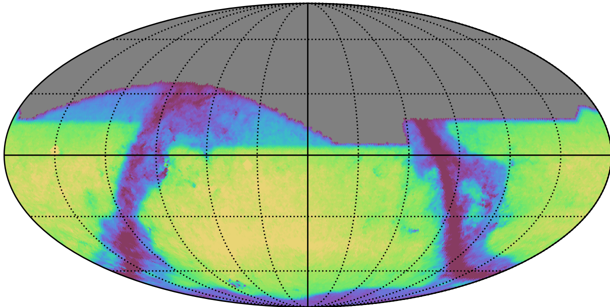
weather_cloudso4v3.5_10yrs i: GalaxyCountsMetricExtended
