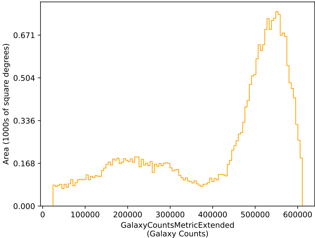
weather_cloudso4v3.5_10yrs r: GalaxyCountsMetricExtended
