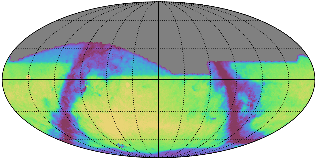
weather_cloudso4v3.5_10yrs r: GalaxyCountsMetricExtended
