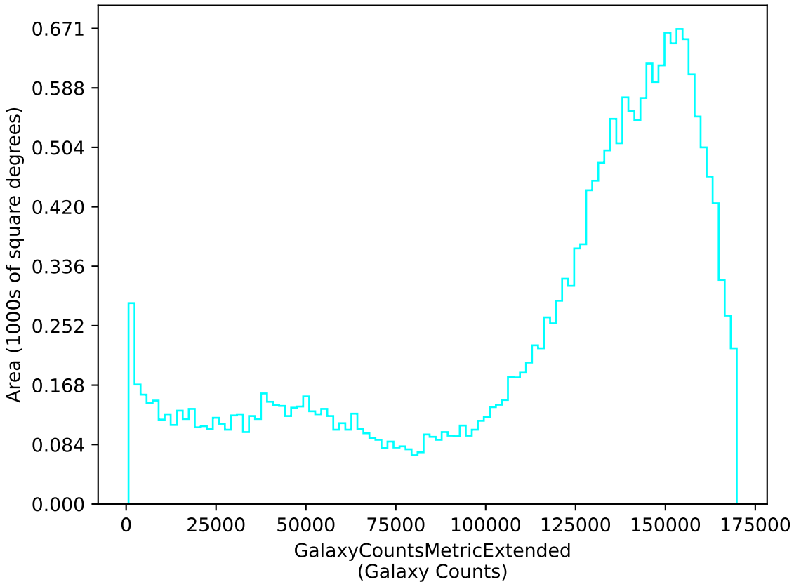
weather_cloudso4v3.5_10yrs u: GalaxyCountsMetricExtended
