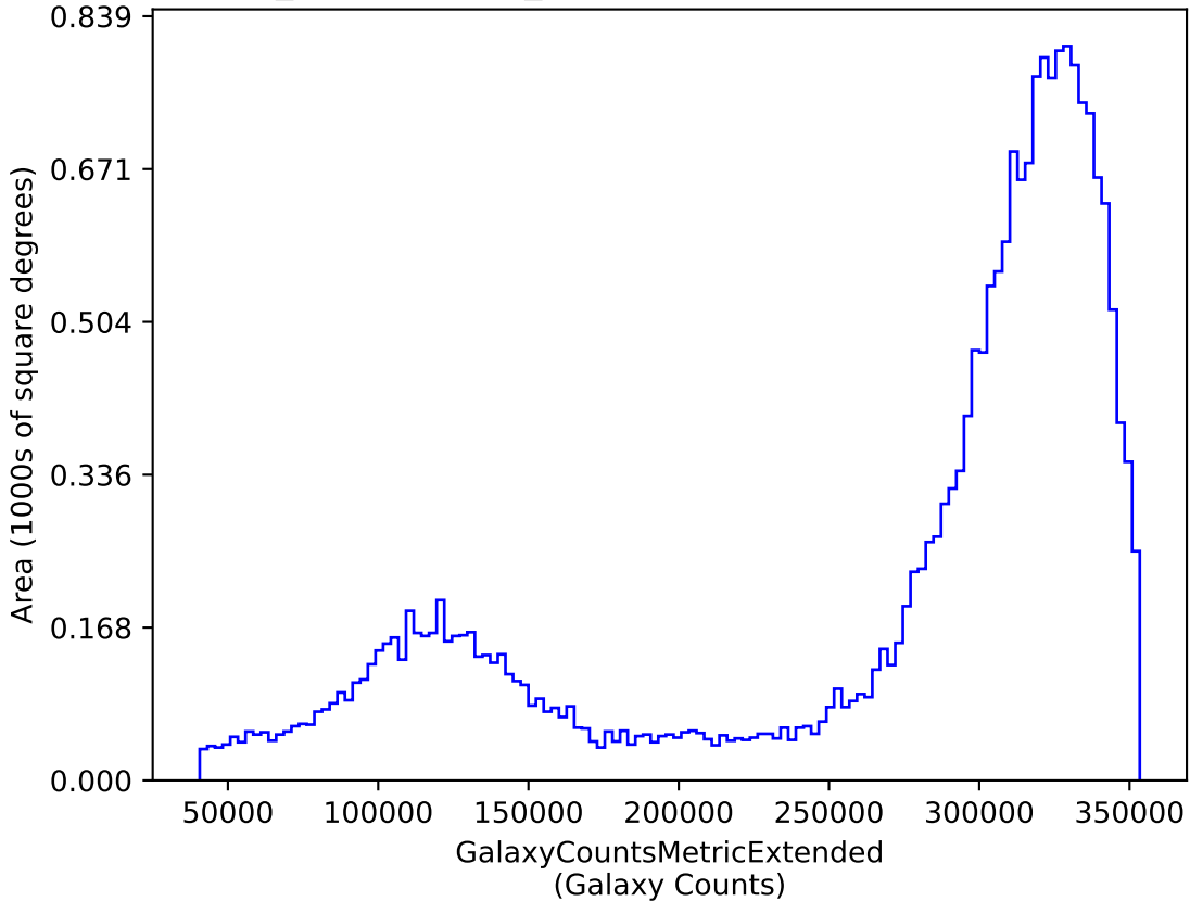
weather_cloudso4v3.5_10yrs y: GalaxyCountsMetricExtended
