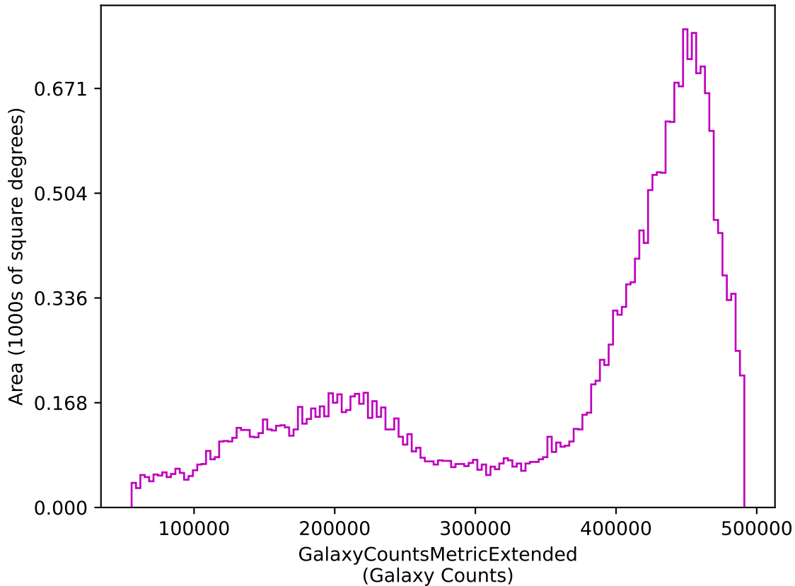
weather_cloudso4v3.5_10yrs z: GalaxyCountsMetricExtended
